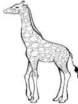
giraffe
