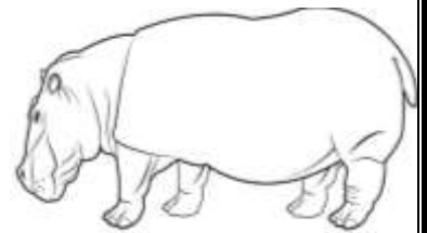
hippopotamus
